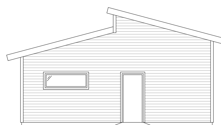
FASAD - GAVEL 1:100
